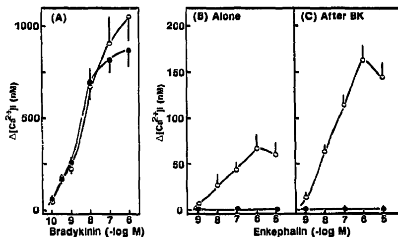
Fig. 2. Effect of PT on dose-response curves of BK and EK-induced [Ca^{2+}]_i rise. The cells were treated without (○) or with (●) PT. Experimental protocols were similar to those for Fig. 1A(a and b) except for the dose of BK or EK. Peak rises in [Ca^{2+}]_i induced by the indicated dose of BK alone (A), EK alone (B), or EK following BK (0.1 nM) (C) are plotted. The results are the means \pm SE of four separate experiments.
