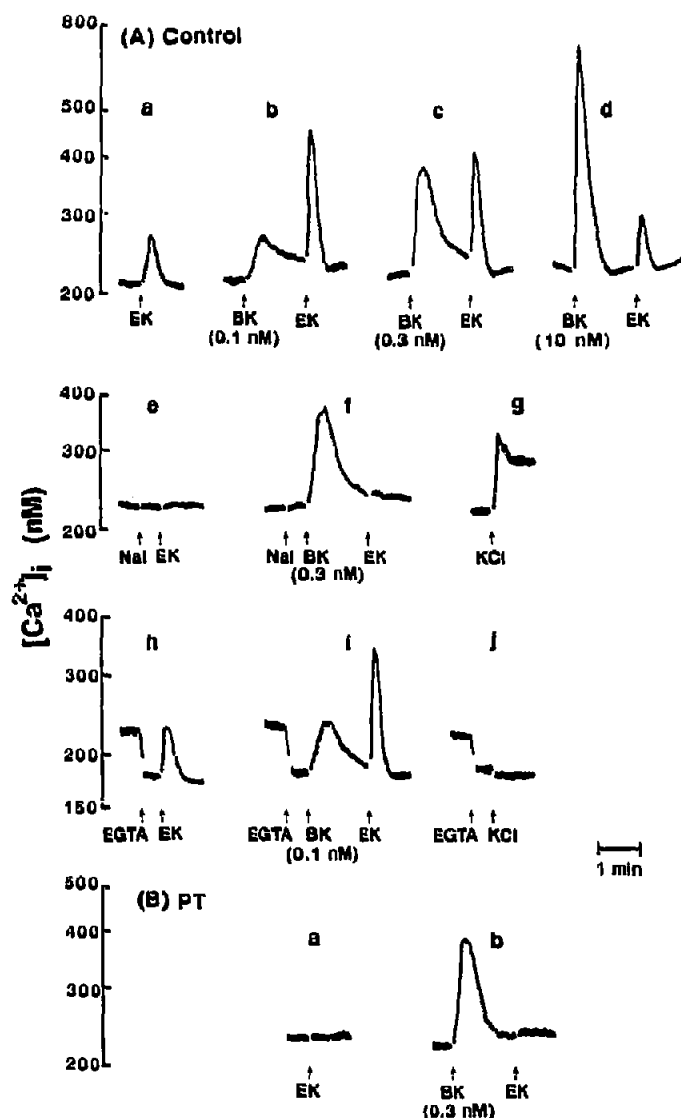
Fig. 1. Effect of EK on [Ca^{2+}]_i in a cell suspension. The cells were treated without (A) or with (B) PT. At arrows, EK ( 1 \mu M ), the indicated dose of BK, naloxone (Nal, 10 \mu M ), KCl ( 50 mM ) and EGTA ( 2.2 mM ) were applied. The representative of at least four separate experiments is shown.
