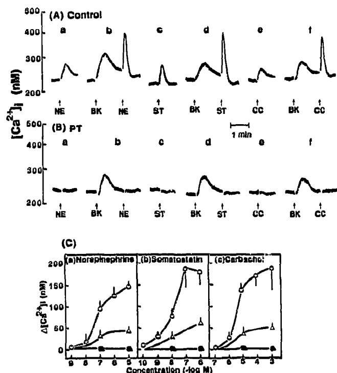
Fig. 3. Effect of norepinephrine, somatostatin and carbachol on [Ca^{2+}]_i . The cells were treated without (A and ○, \Delta in C) or with (B and ●, \blacktriangle in C) PT. Experimental conditions were the same as those for Figs. 1 and 2. In A and B, at arrows, EK (1 \mu M), BK (0.1 nM), norepinephrine (NE, 1 \mu M), somatostatin (ST, 100 nM) and carbachol (CC, 100 \mu M) were applied. The representative of at least four separate experiments is shown. In C, peak rises in [Ca^{2+}]_i induced by the indicated dose of norepinephrine (a), somatostatin (b) or carbachol (c) alone ( \Delta , \blacktriangle ) or these agonists following BK (○, ●) are plotted. The results are the means \pm SE of four separate experiments.
